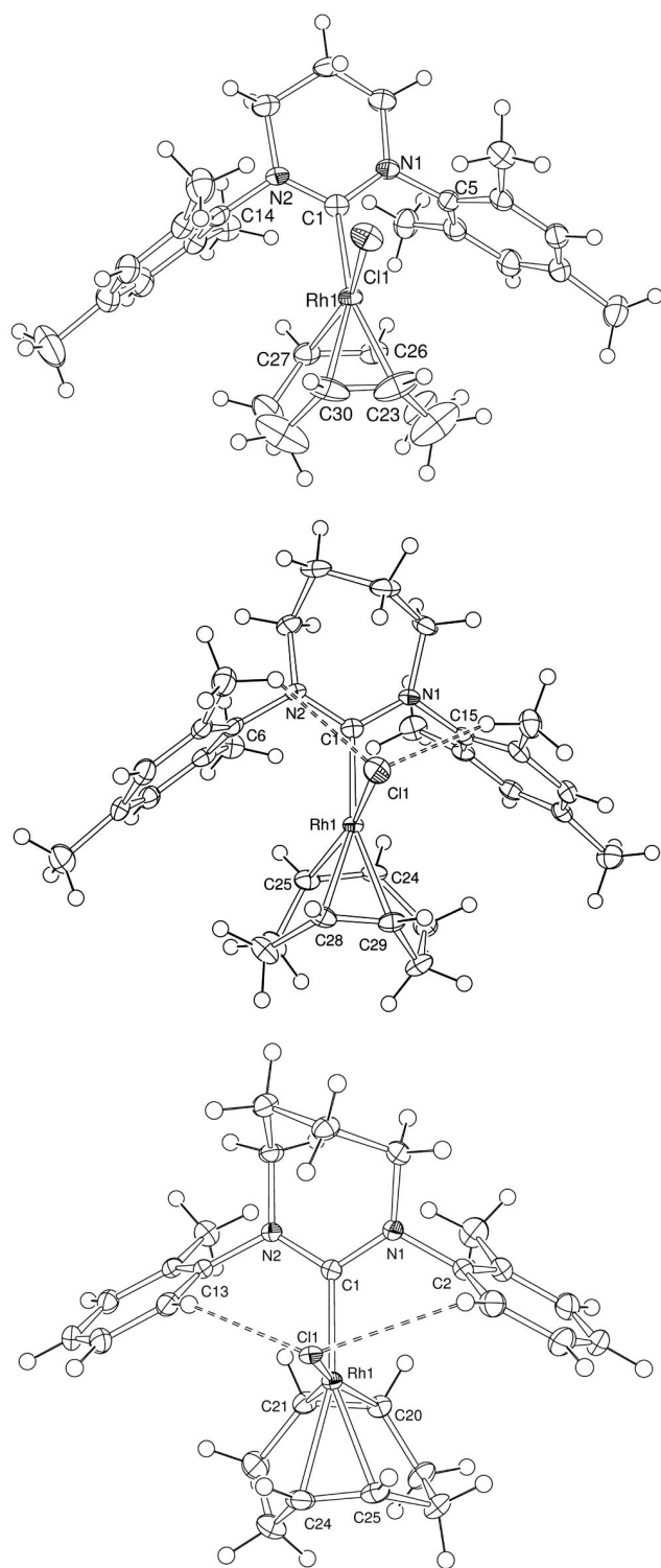
Figure 1. Solid-state molecular structures of Rh(6-Mes)(COD)Cl, Rh(7-Mes)(COD)Cl and Rh(7- o Tol)(COD)Cl.
