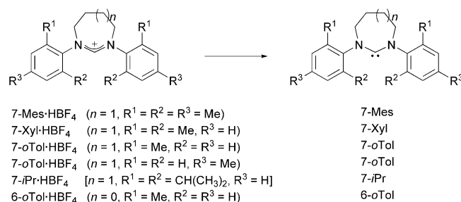
Scheme 2. Synthesis of six- and seven-membered NHCs with N-aryl substituents. Reagents and conditions: \text{KN}(\text{SiMe}_3)_2 , thf.
