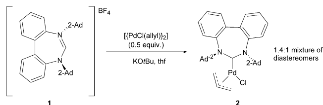
Scheme 1. Synthesis of Stahl's \text{Pd}^{\text{II}} carbene complex.
