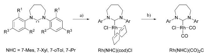
Scheme 3. Synthesis of \text{Rh}(\text{NHC})(\text{COD})\text{Cl} and \text{Rh}(\text{NHC})(\text{CO})_2\text{Cl} complexes. (a) [\text{Rh}(\text{cod})\text{Cl}]_2 , thf; (b) CO (1 atm), \text{CH}_2\text{Cl}_2 .
