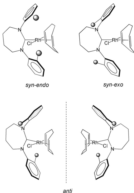
Scheme 4. Rotamers of \text{Rh}(7\text{-}o\text{Tol})(\text{COD})\text{Cl} .
